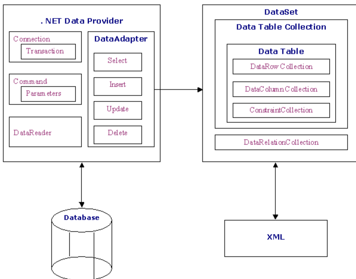
ADO .NET Data Architecture
